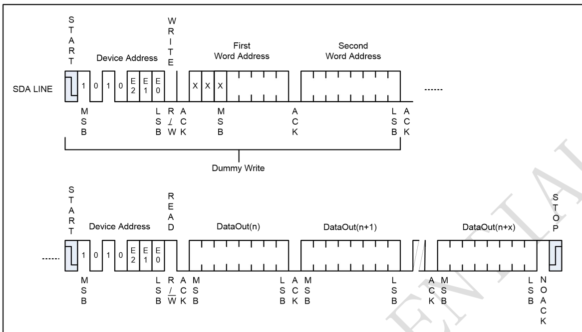
Figure 5-5 Sequential Read
