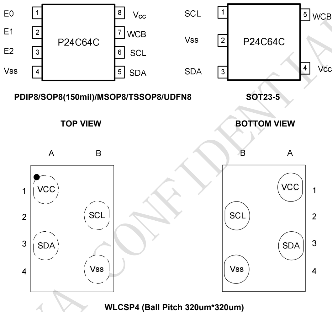
Figure 1-1 Pin Configuration
