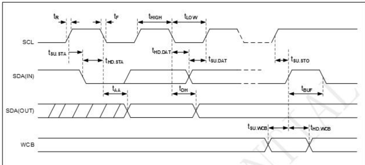
Figure 3-1 Bus Timing
